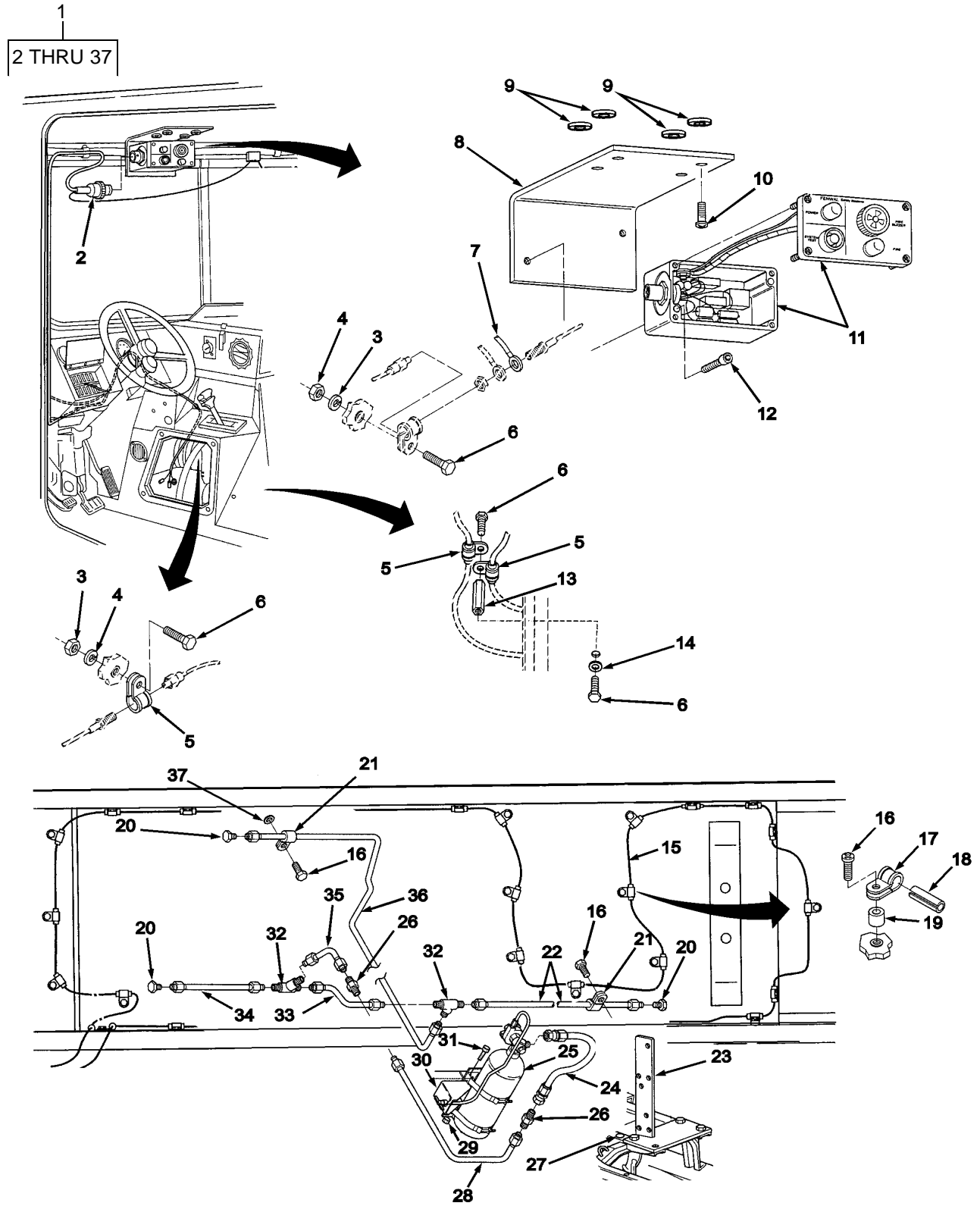
FIGURE 231. ENGINE FIRE SUPPRESSION KIT.
