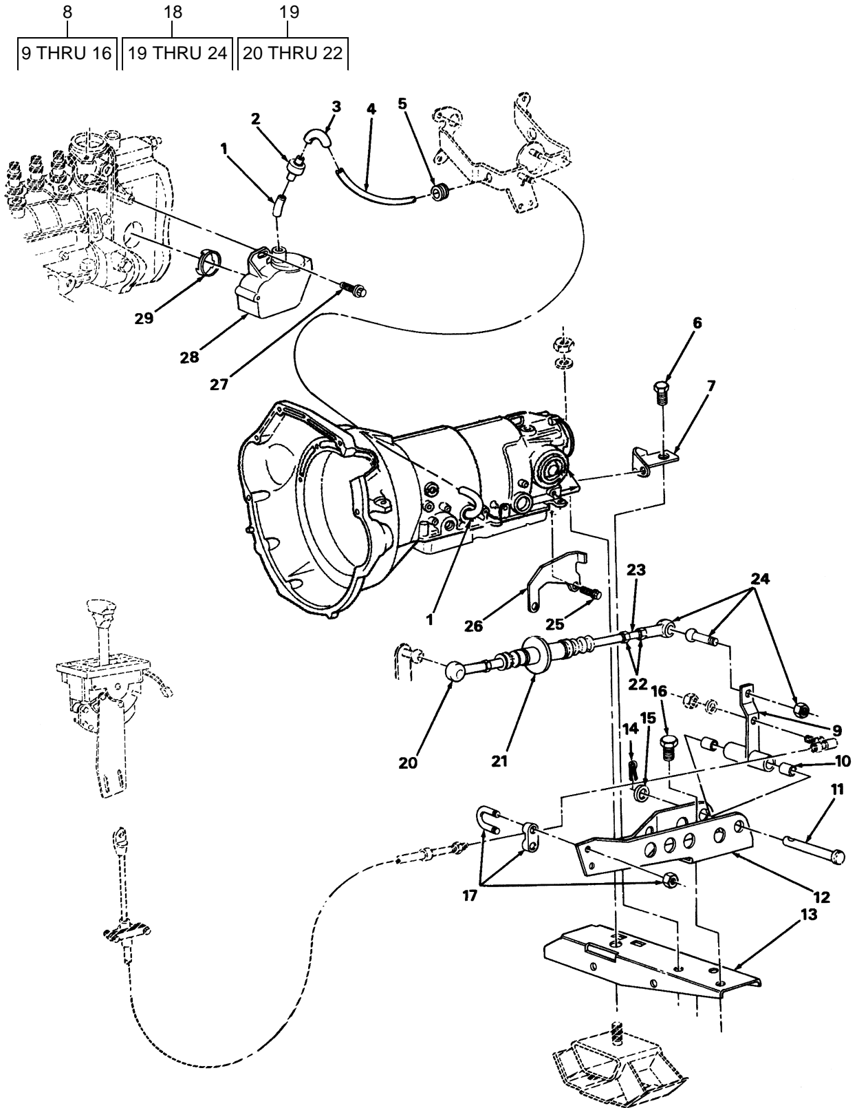
FIGURE 102. SHIFT LINKAGE, MOUNTS, VACUUM VALVE, AND RELATED PARTS.
