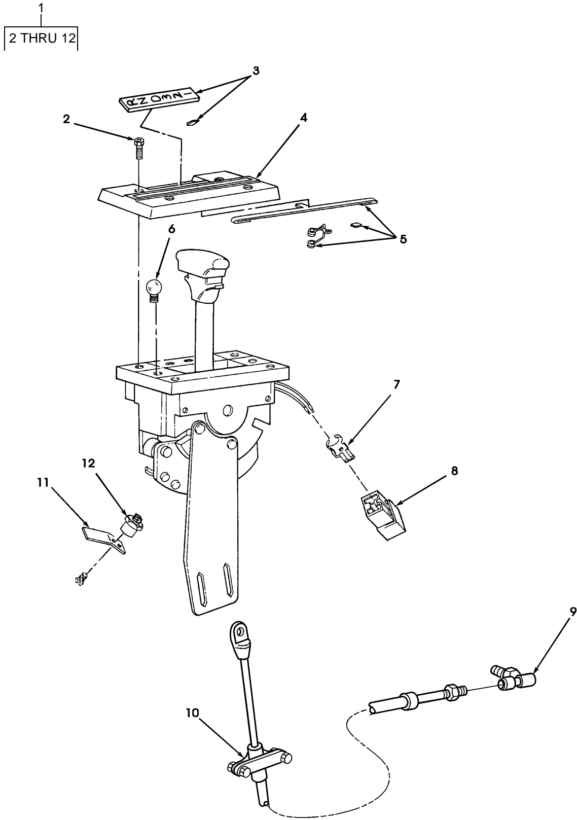
FIGURE 101. SHIFTER ASSEMBLY.
