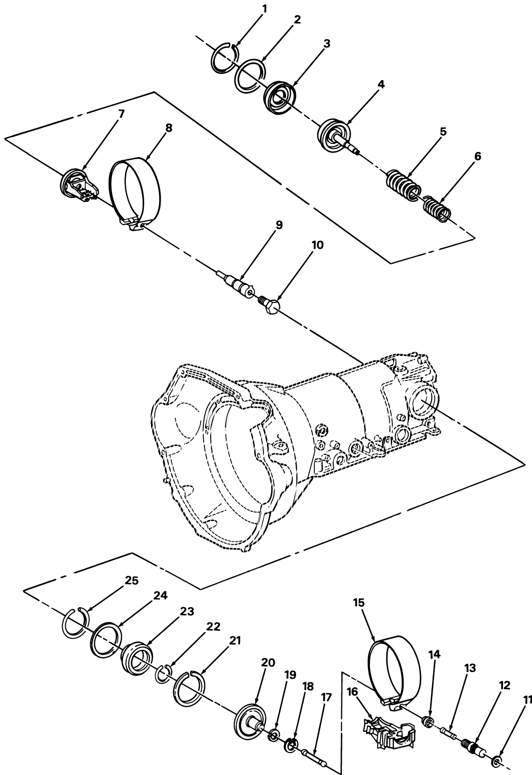
FIGURE 116. BRAKE BANDS AND SERVO.
