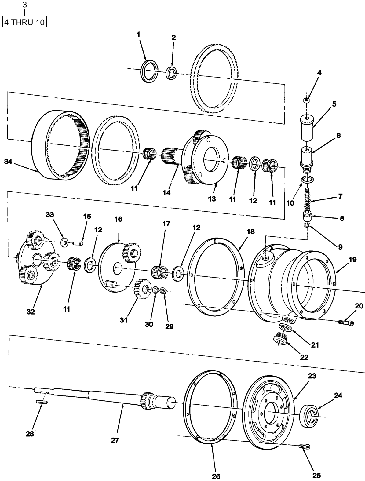
FIGURE 199. PLANETARY GEARS AND HOUSING.
