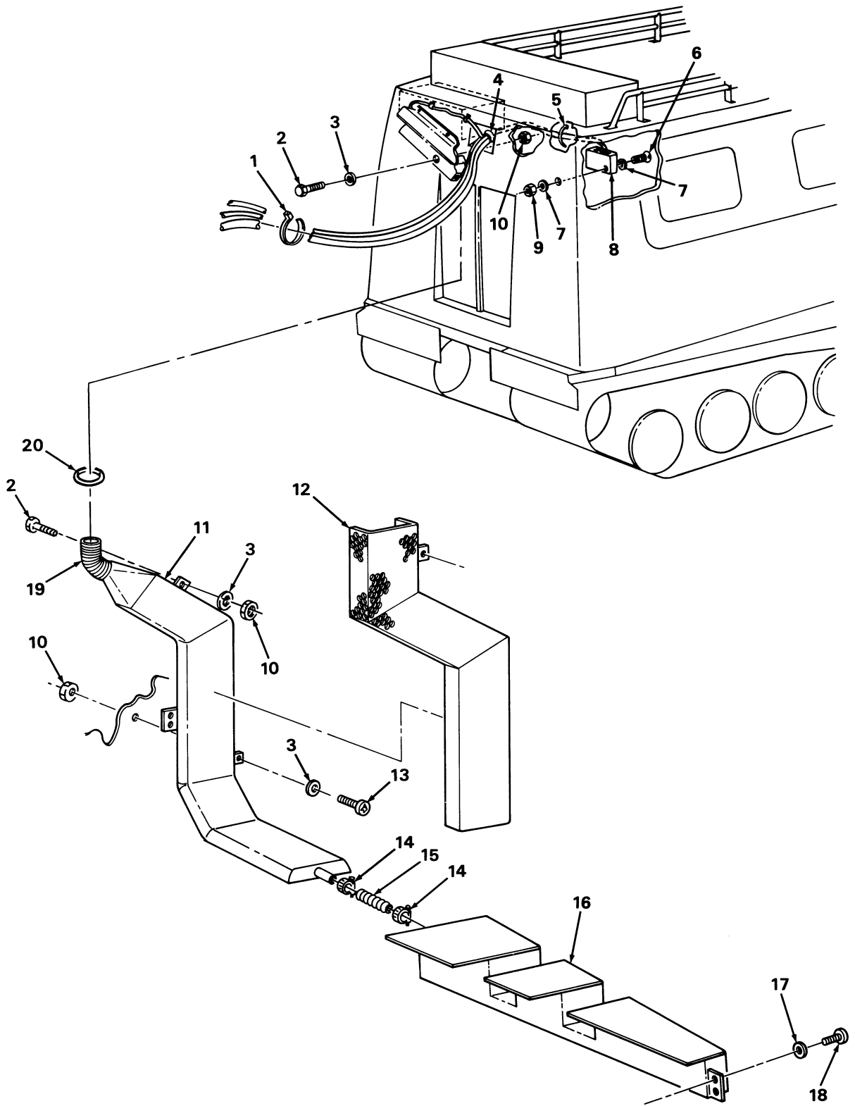
FIGURE 215. HEATER AIR PASSAGE ASSEMBLY.
