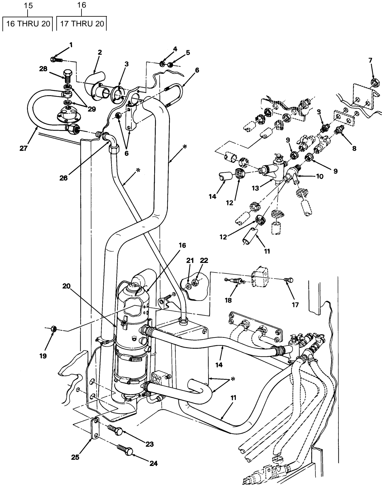
FIGURE 223. WATER HEATER HOSES AND RELATED PARTS.
