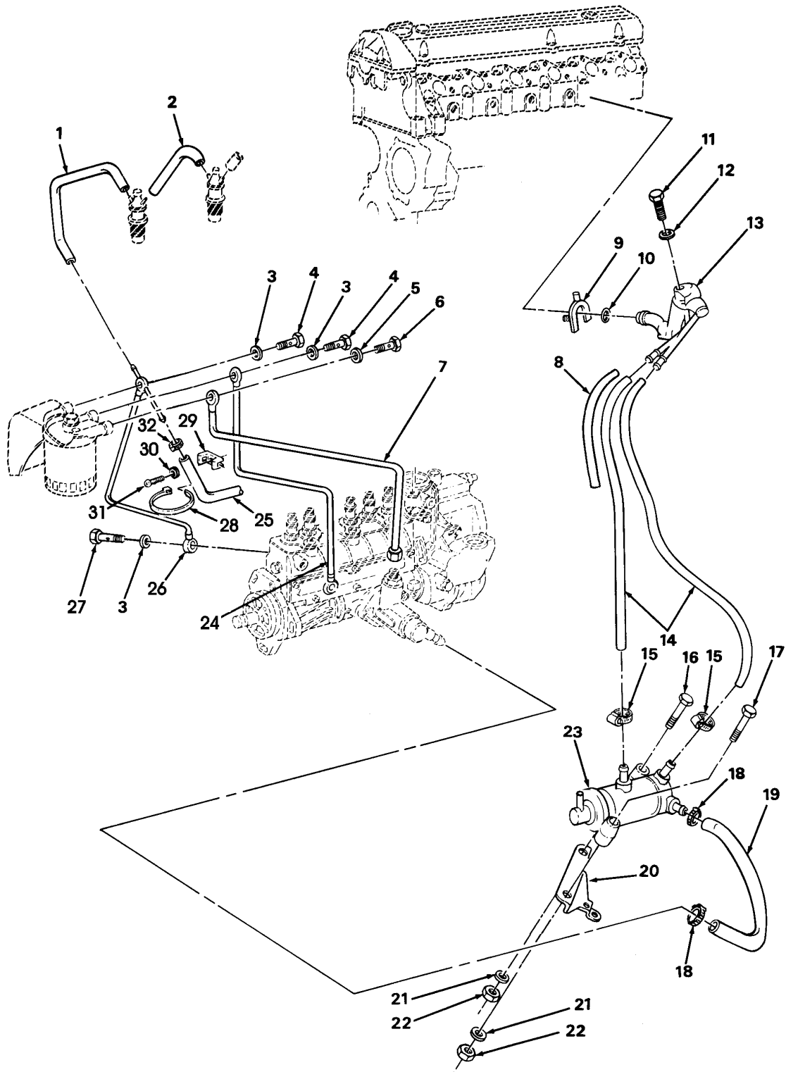
FIGURE 21. FUEL INJECTION PUMP LINES AND RELATED PARTS.
