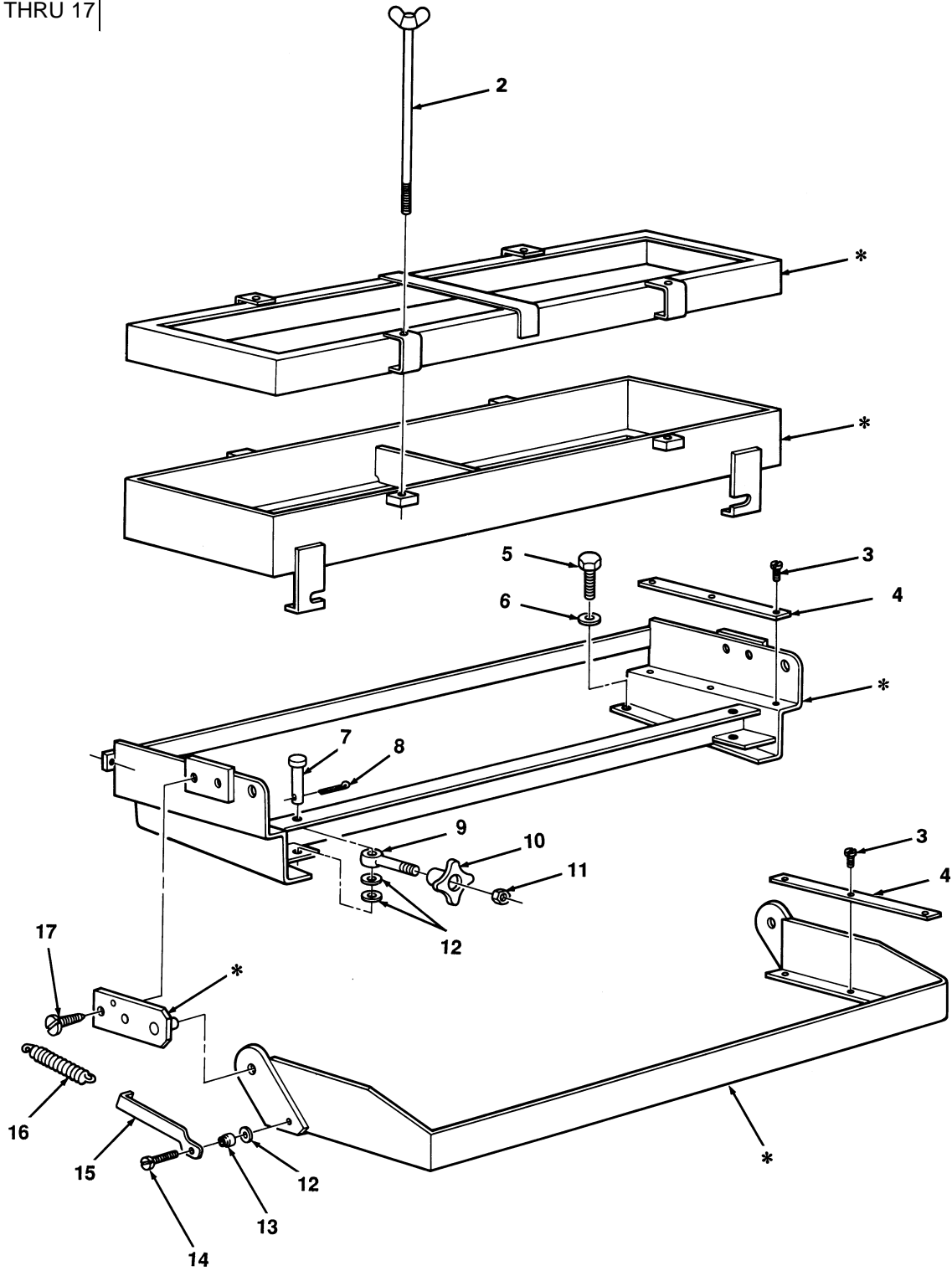
FIGURE 87. BATTERY BOX, REAR CAR.
