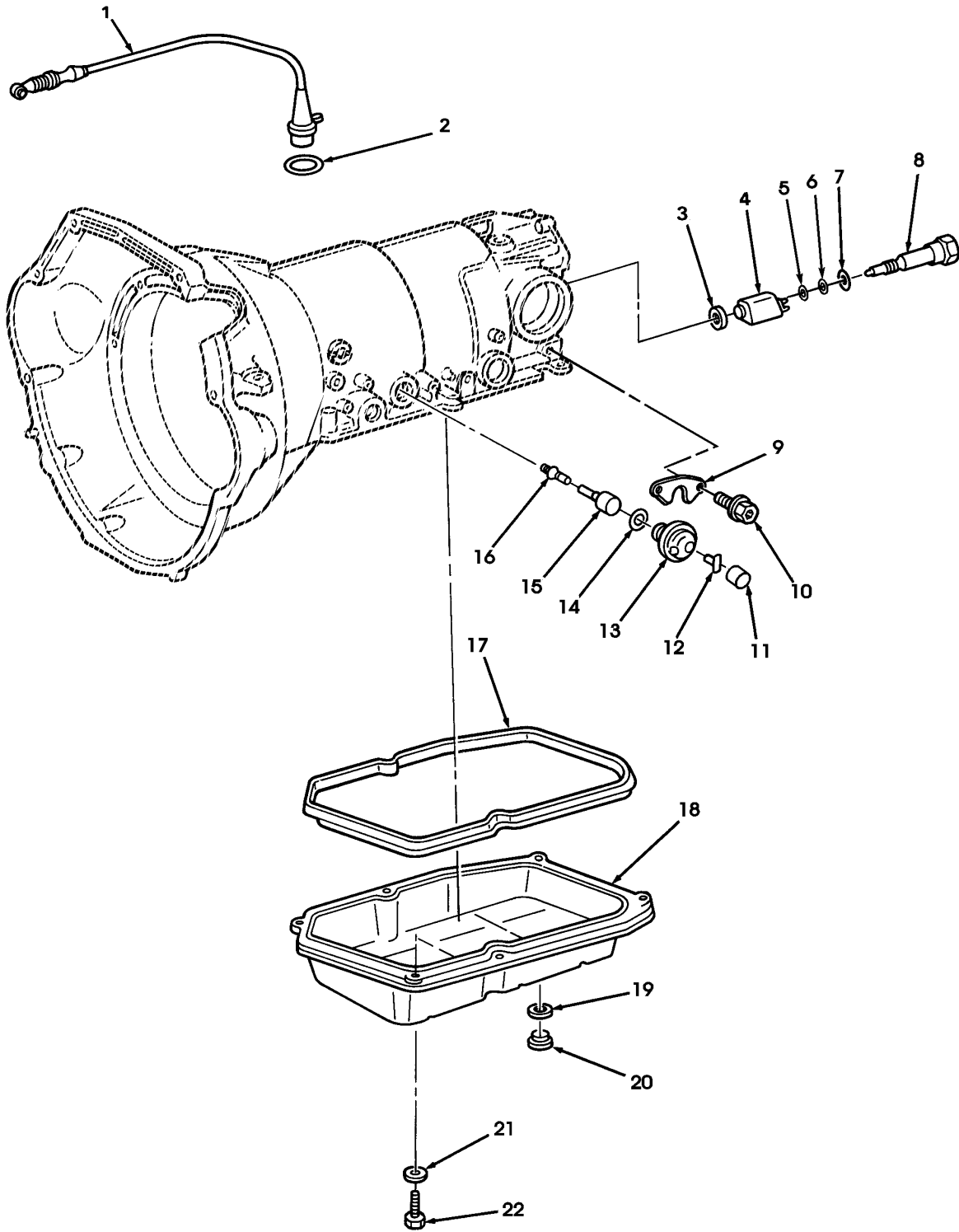
FIGURE 106. CONTROL ASSEMBLY, COIL, DETENT PLUNGER, DIAPHRAGM, AND OIL PAN.
