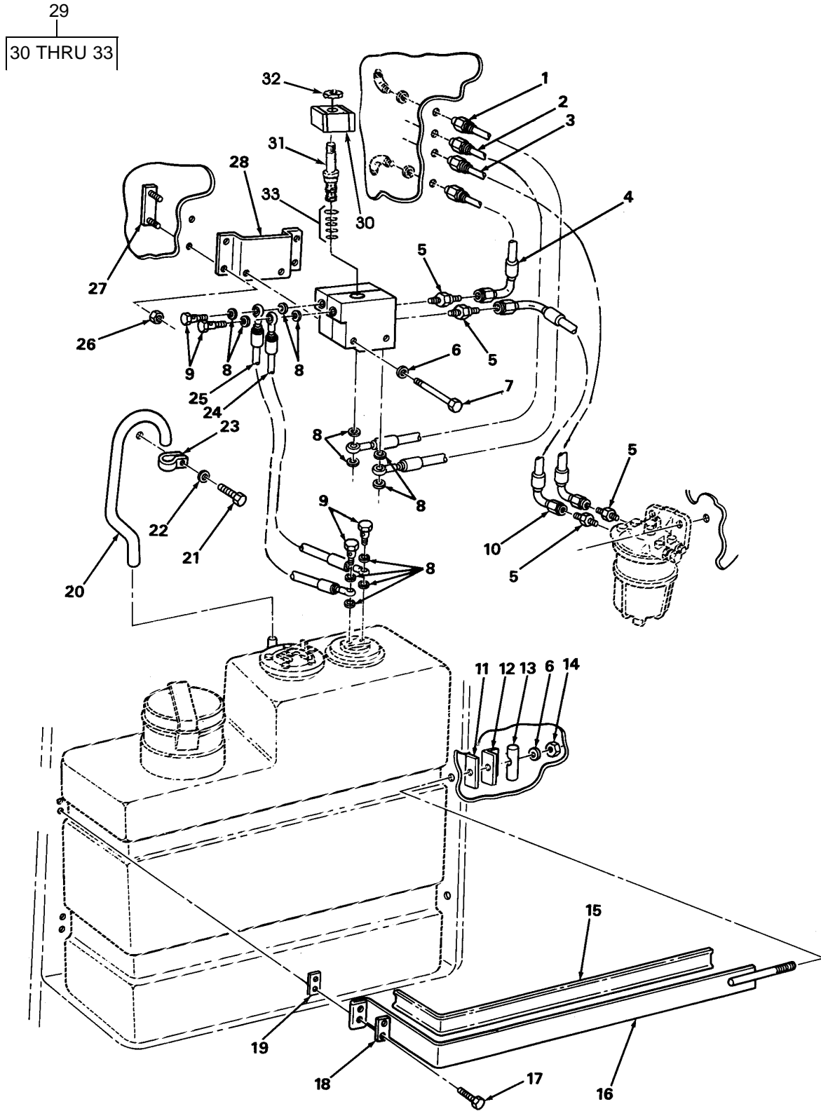
FIGURE 25. LEFT FUEL TANK LINES, FITTINGS, AND MOUNTING PARTS.
