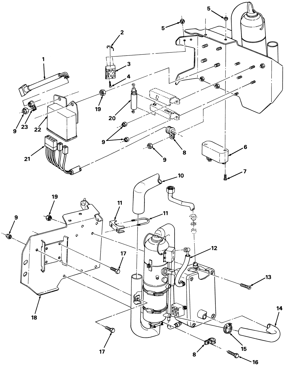
FIGURE 224. WATER HEATER ASSEMBLY.
