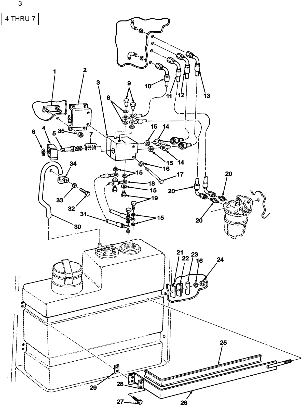
FIGURE 26. LEFT FUEL TANK LINES, FITTINGS, AND MOUNTING PARTS.
