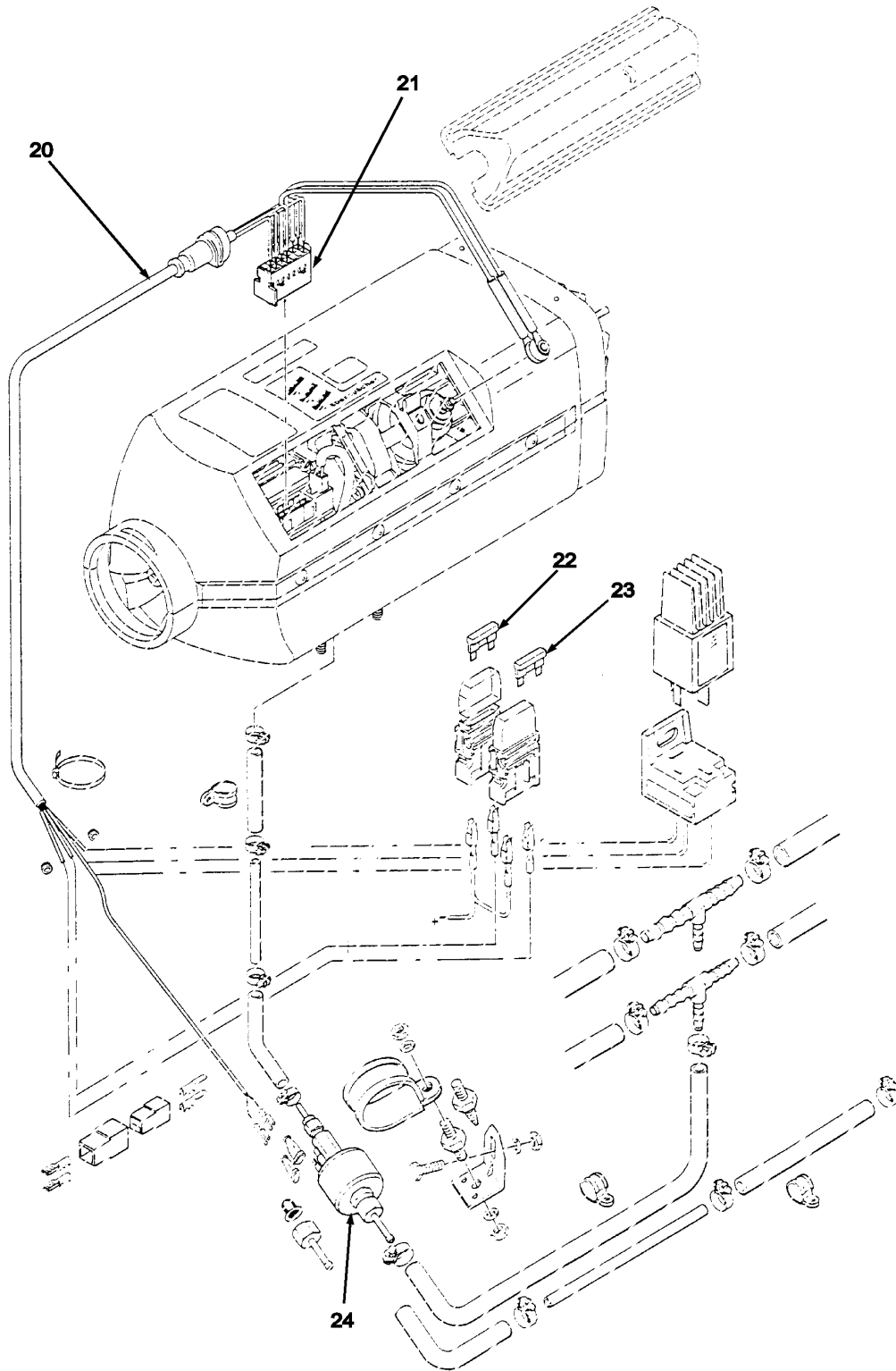
FIGURE 216. AMBULANCE REAR CAR HEATER (SHEET 2 OF 4).
