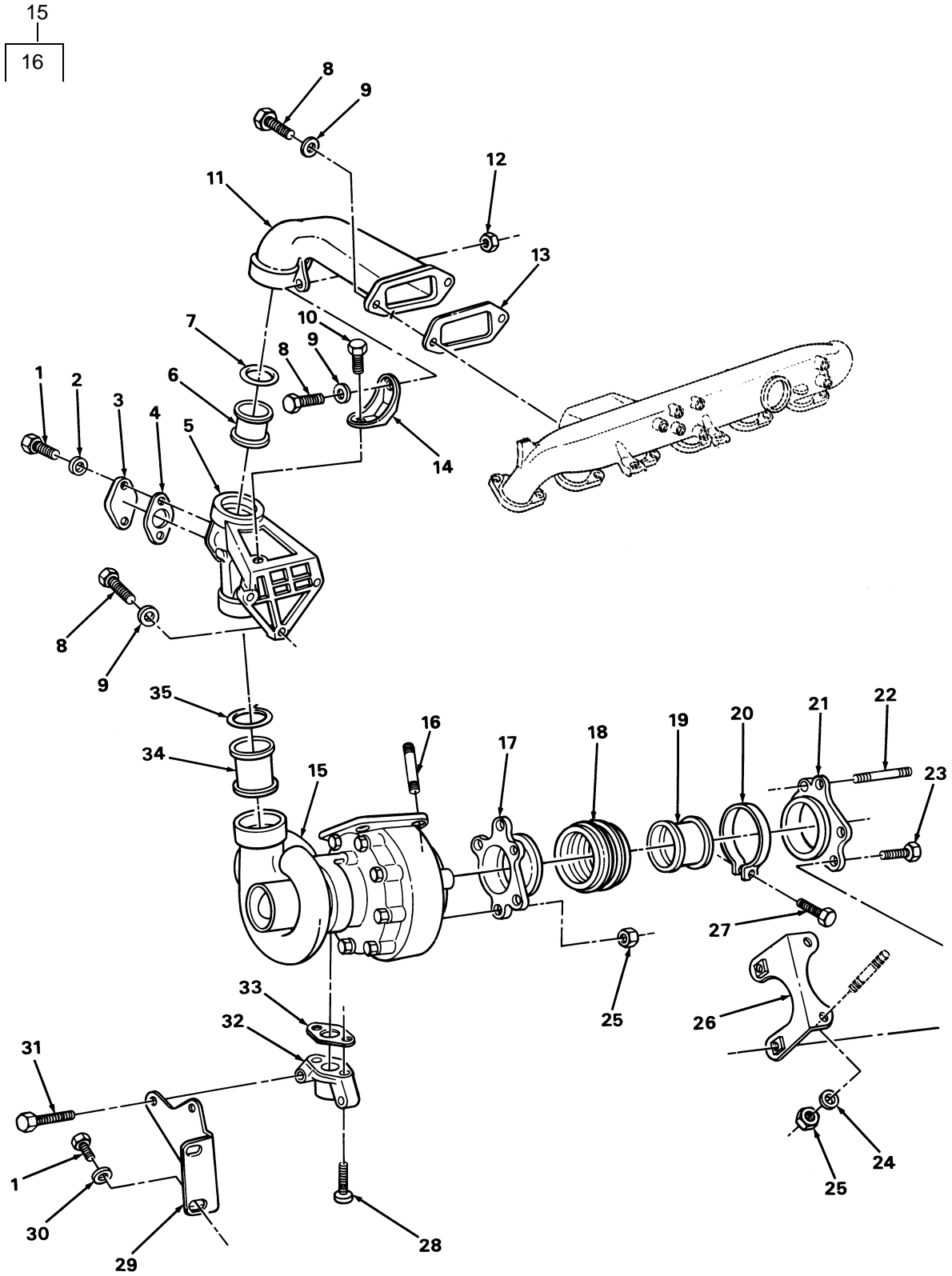
FIGURE 20. TURBOCHARGER AND RELATED PARTS.
