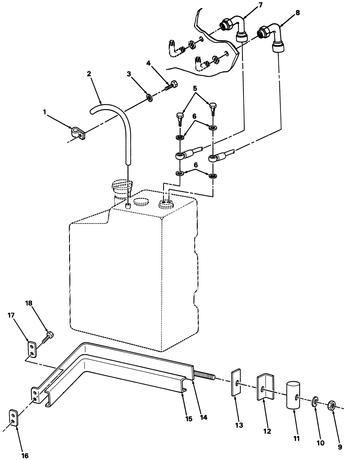
FIGURE 24. RIGHT FUEL TANK LINES, FITTINGS, AND MOUNTING PARTS.
