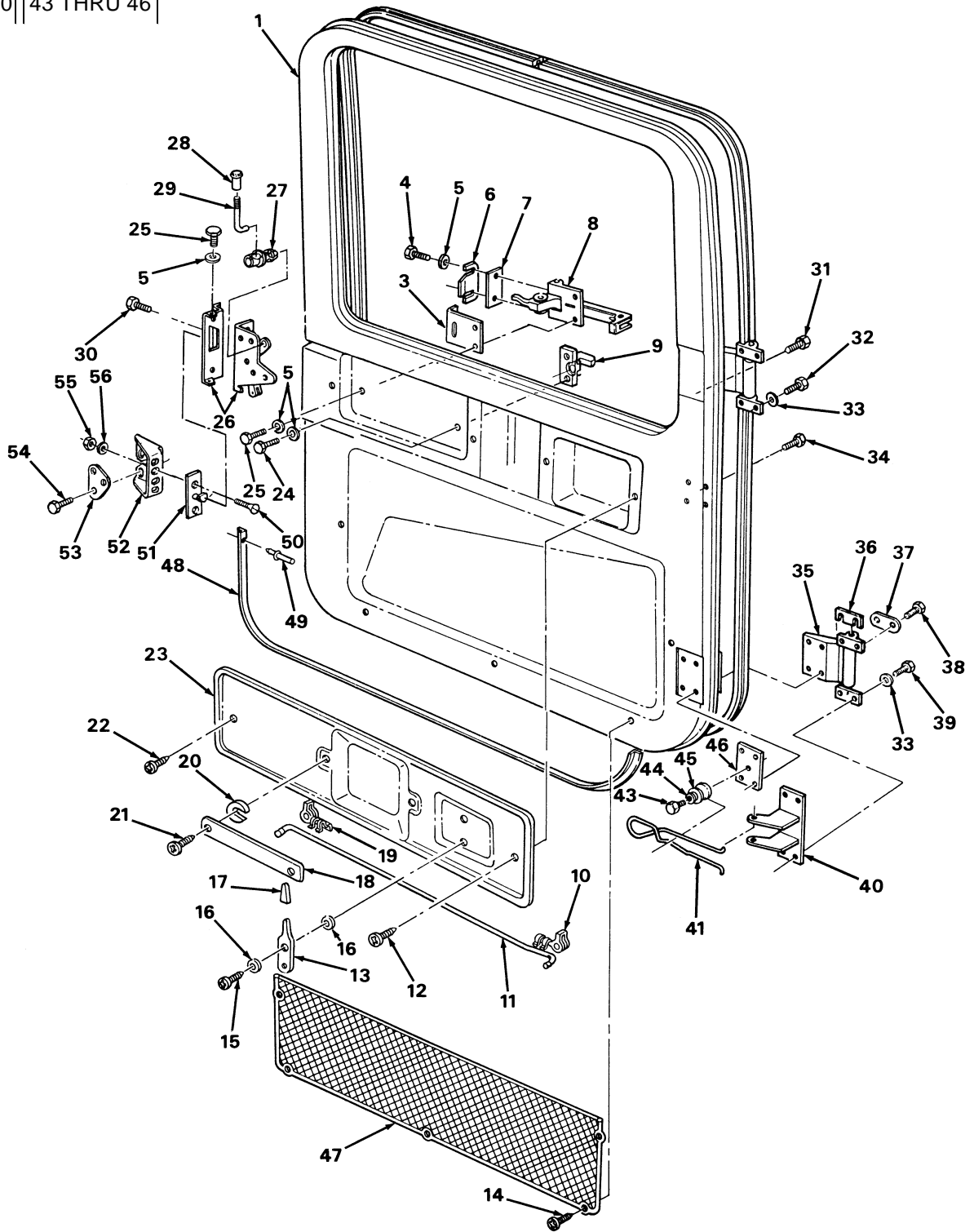
FIGURE 156. FRONT CAR HATCH DOORS.
