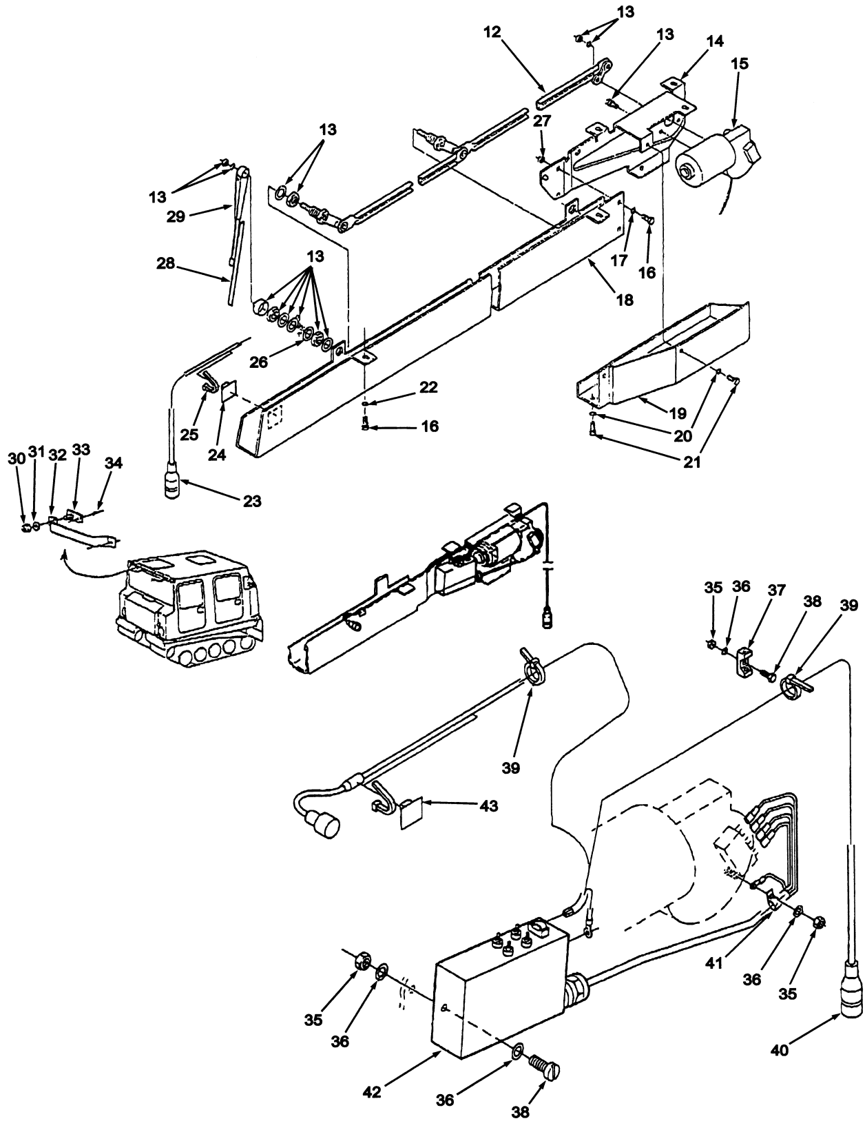
FIGURE 208. WINDSHIELD WIPER ASSEMBLY (SHEET 2 OF 2).
