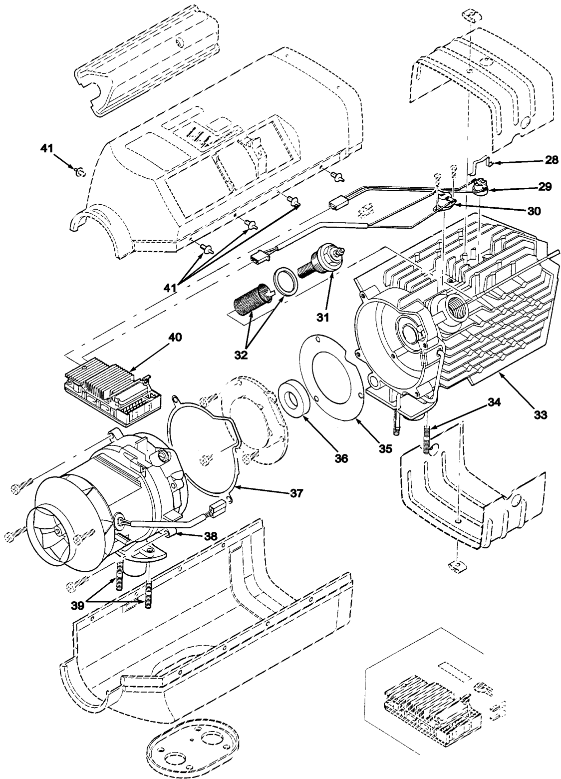
FIGURE 216. AMBULANCE REAR CAR HEATER (SHEET 4 OF 4).
