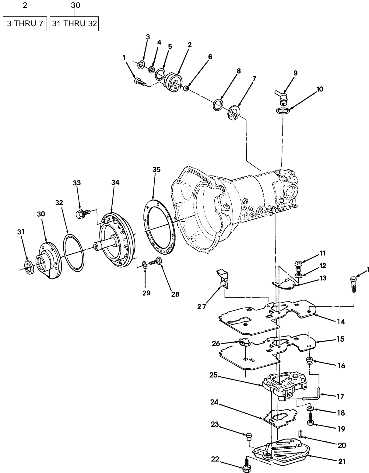
FIGURE 118. PRIMARY AND SECONDARY OIL PUMPS, OIL FILTER, AND COVER, AND BREATHER VALVE.
