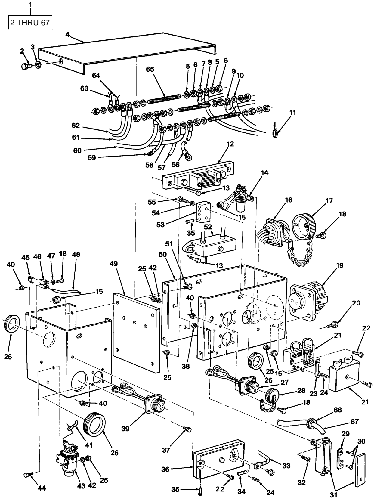
FIGURE 53. CONNECTION BOX AND COMPONENT PARTS.
