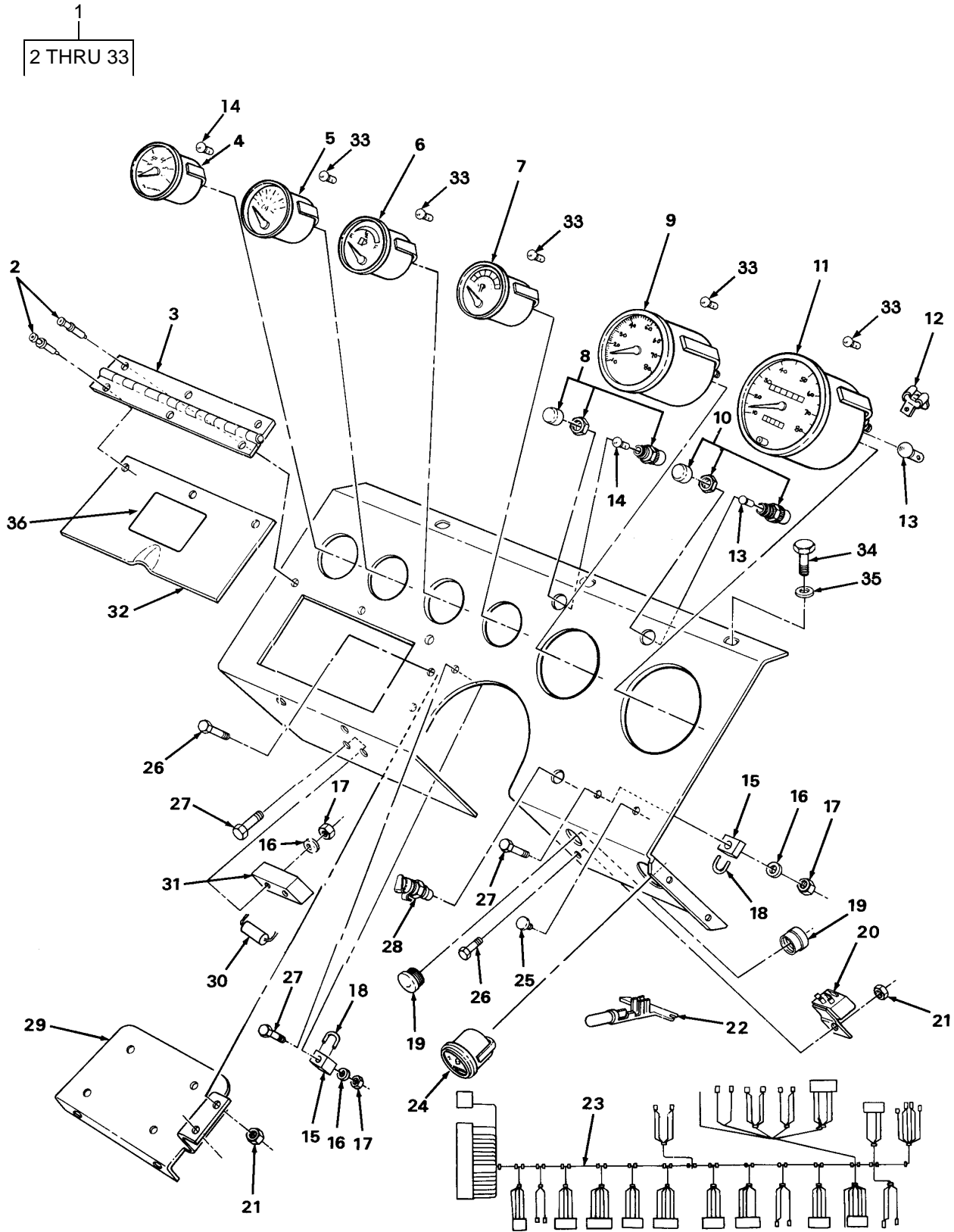
FIGURE 46. INSTRUMENT PANEL AND COMPONENT PARTS.
